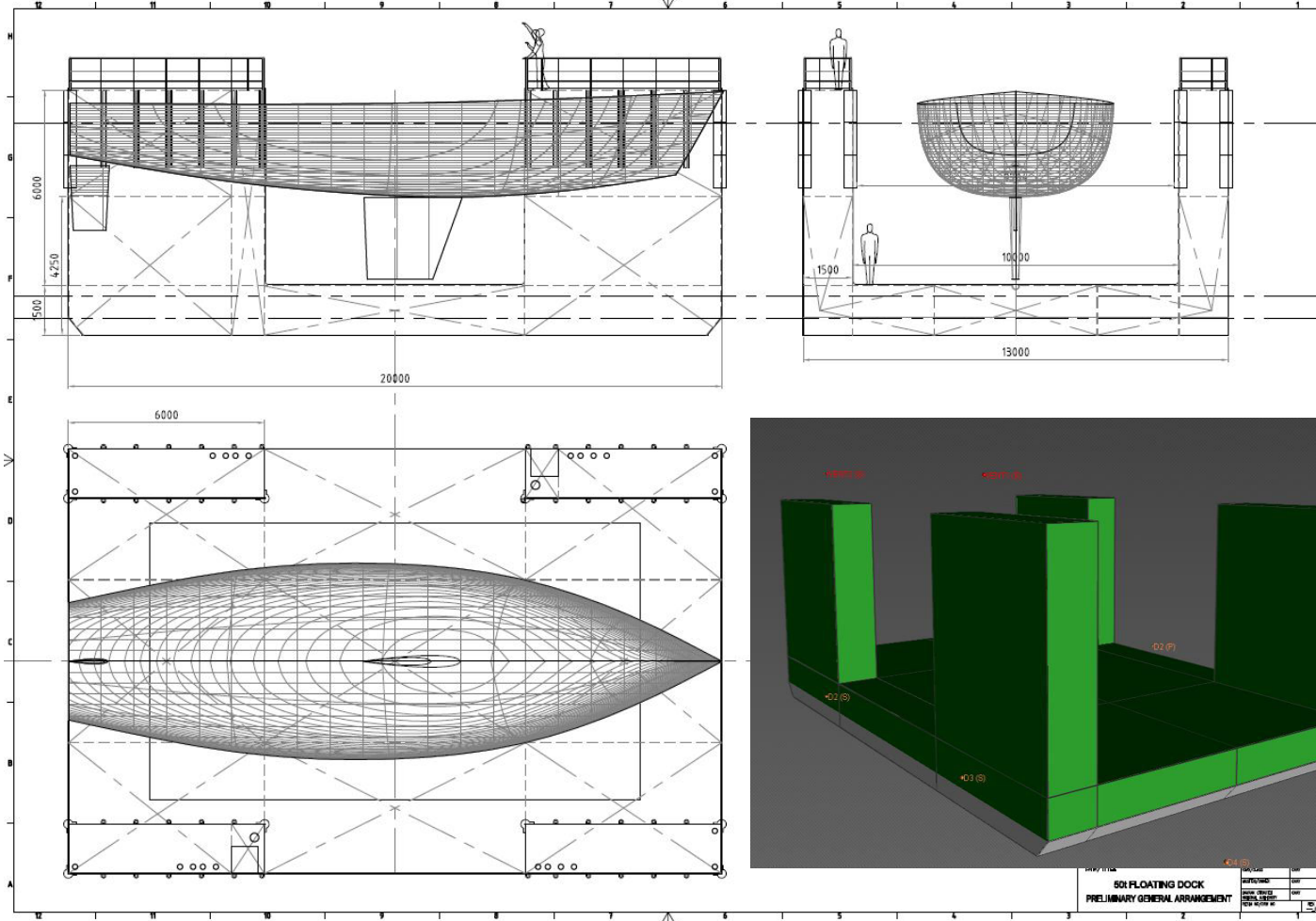
Floating Docks for Yachts/Workboats
