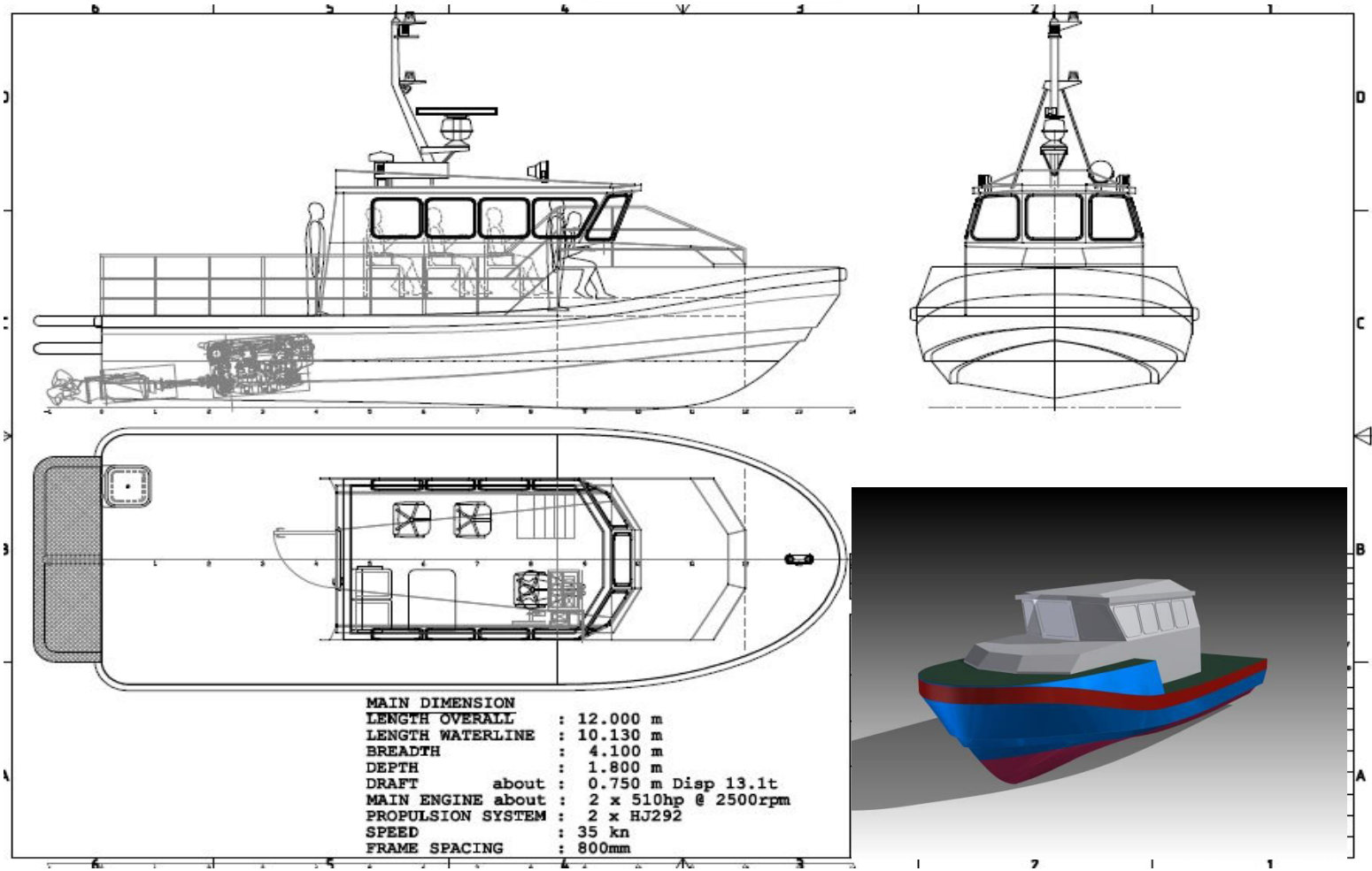
SAR Boats / Patrol Boats
